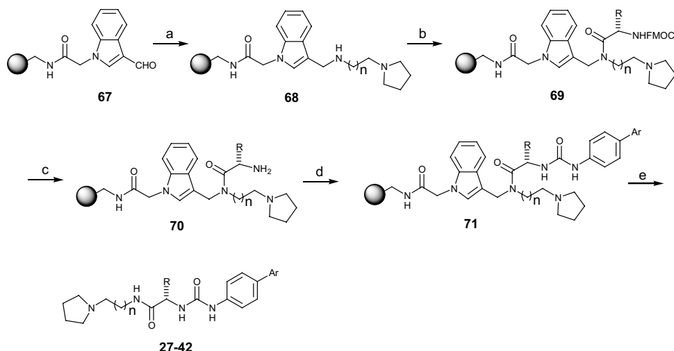
Scheme 3. Reagents: (a) appropriate amine, \text{Ti}(\text{iPrO})_4 , \text{NaBH}_4 , EtOH; (b) appropriate Fmoc-amino acid, DIC, DMAP; (c) 20% Piperidine, DMF; (d) \text{ArPhNCO} , \text{CH}_2\text{Cl}_2 , DMF; (e) 50% \text{CF}_3\text{CO}_2\text{H} , \text{CH}_2\text{Cl}_2 .
