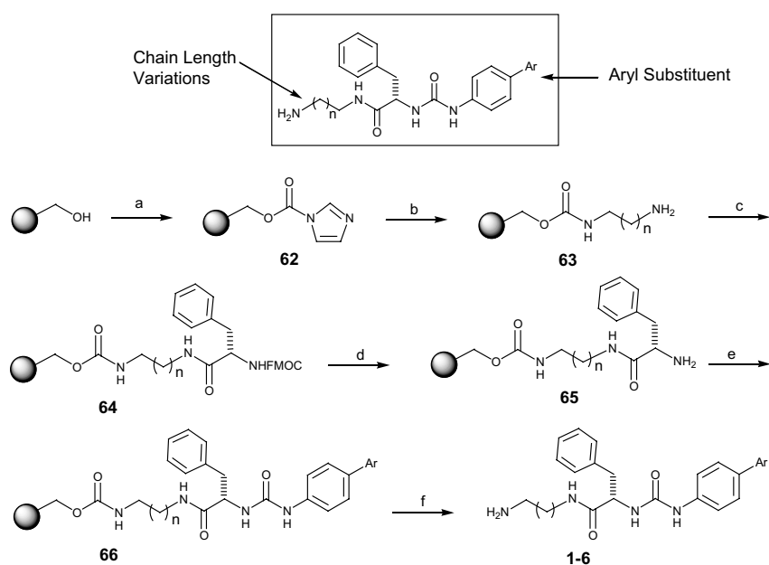
Scheme 2. Reagents: Only phenylalanine is illustrated for clarity (a) Wang resin, carbonyl diimidazole, THF; (b) ethylene diamine or 1,3-diaminopropane, DIPEA, CH 2 Cl 2 ; (c) N -FMOC-Phe, diisopropyl carbodiimide, DMAP, 20% DMF/CH 2 Cl 2 ; (d) 20% Piperidine, DMF; (e) ArPhNCO, DMF/CH 2 Cl 2 (20:80 v/v); (f) CF 3 CO 2 H, CH 2 Cl 2 .
