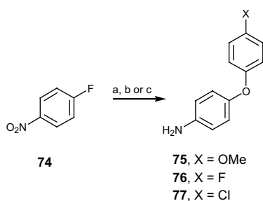
Scheme 5. Reagents: (a) appropriate phenol, \text{Cs}_2\text{CO}_3 , DMA; (b) \text{H}_2/\text{Pd-C} , EtOH; (c) \text{Na}_2\text{S}_2\text{O}_4 , \text{THF}\cdot\text{H}_2\text{O} (3:1, v/v).
